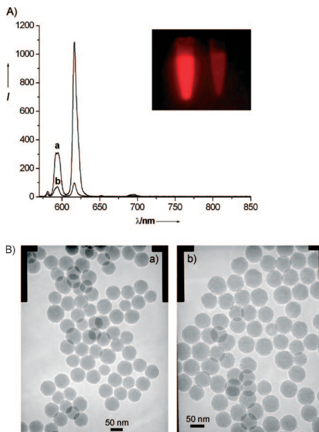
Figure 1. A) Fluorescence spectra of a) Sensor 1 and b) Sensor 2 in the presence of 1\ \mu\text{M} CaDPA at pH 6.5. The inset shows visual fluorescence color of Sensor 1 (left) and Sensor 2 (right) in the presence of 10\ \mu\text{M} CaDPA (filtration with a CB565 filter). B) TEM images of FITC-doped silica nanoparticles a) without and b) with the sensing moiety.
